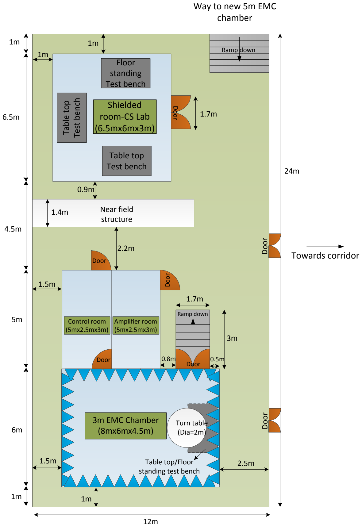
Plan diagram of EMC CHAMBER and CS LAB in the existing 24×12×5.5m RCC BUILDING:
